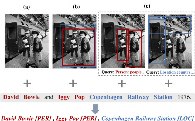
Figure 1: An example for multimodal named entity recognition with (a) the whole image cue, (b) region cues from VG toolkit, (c) region cues paired with queries for entity types.
